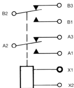
SCHEMATIC DIAGRAM
