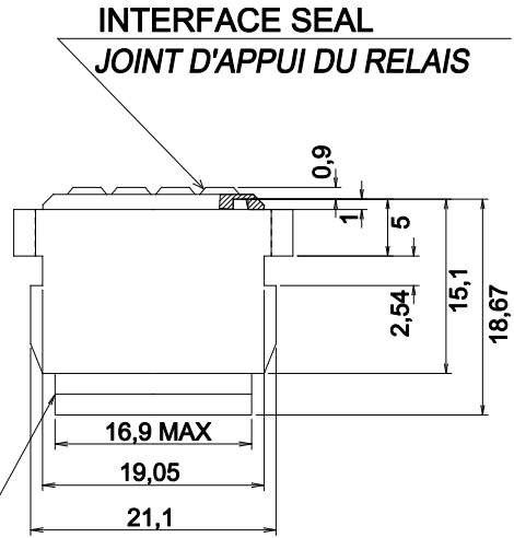
WIRE SEALING GROMMET JOINT D'ETANCHEITE
